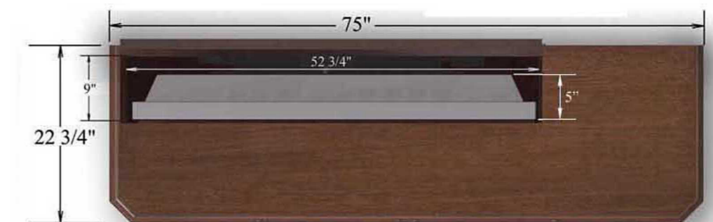
TOP VIEW (Closed)
