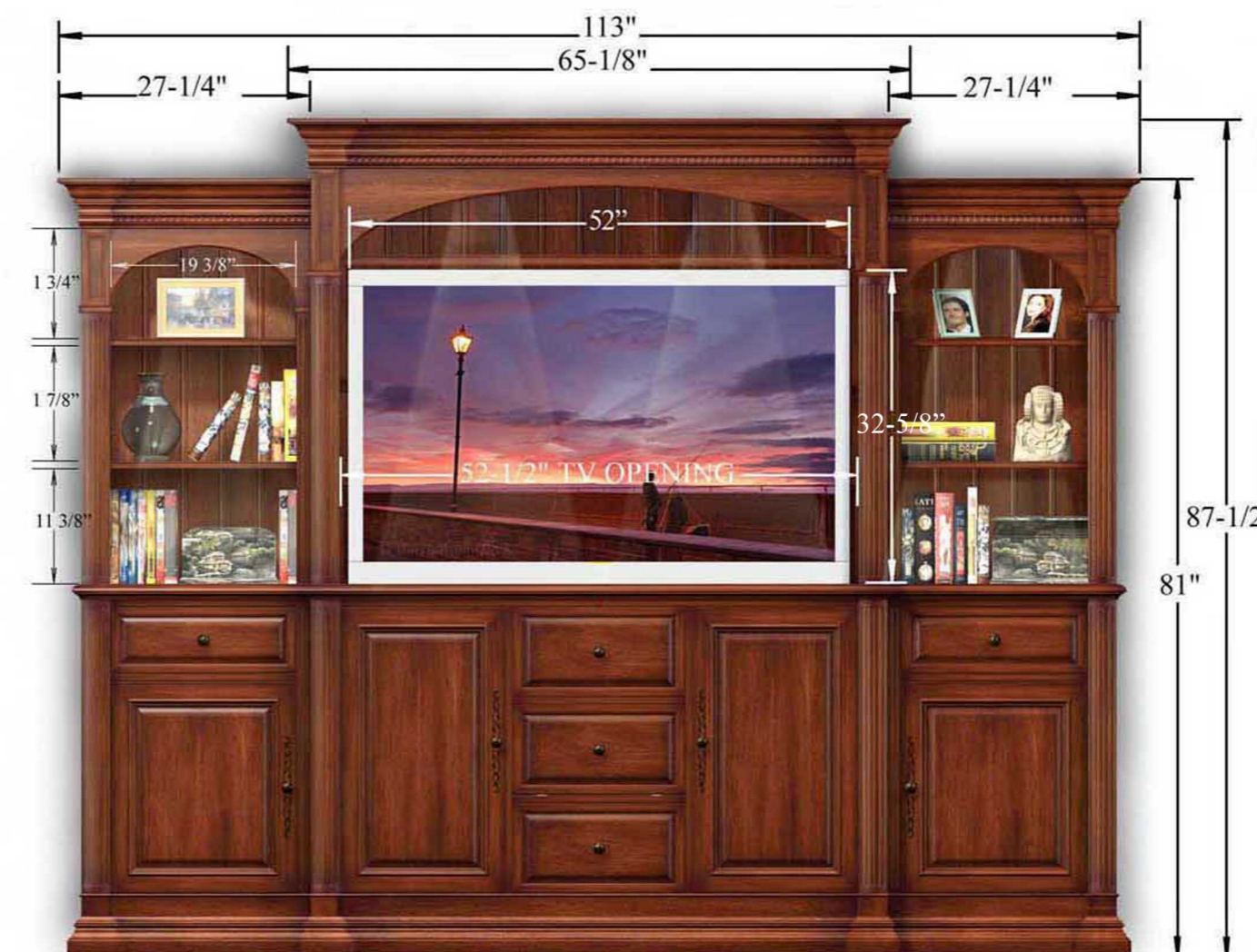
FRONT VIEW (open)
