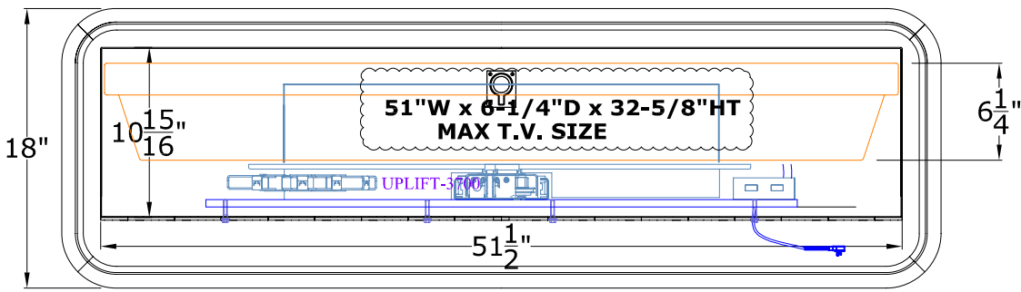
TOP VIEW
