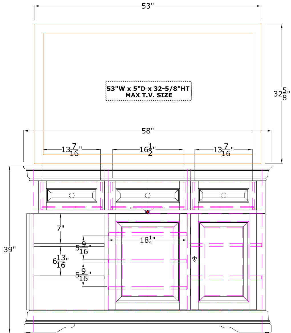
FRONT VIEW
