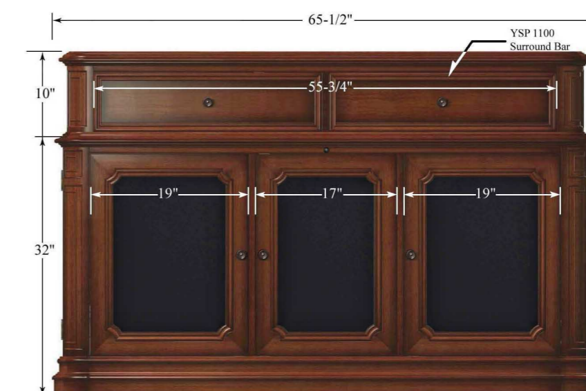
FRONT VIEW (shown with speaker cloth option on doors and wooden panel option on top drawers)
