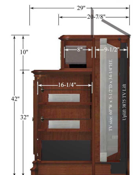
SIDE SECTION
