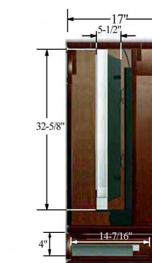
SIDE SECTION
